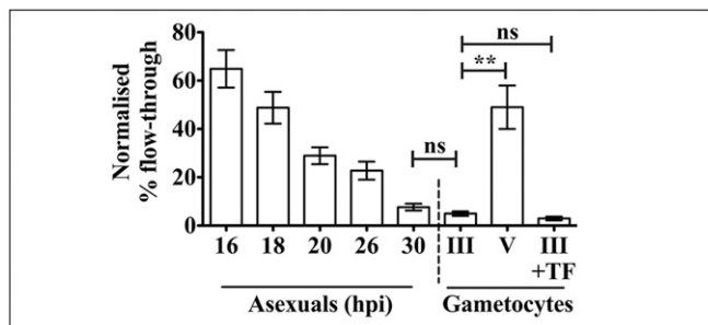
Fig. 1. Filterability of asexual and sexual P. falciparum and effect of microtubule destabilization. Asexual stage-infected RBCs at different hours after invasion, stage III (day 6) gametocytes (with or without 24-h trifluralin treatment) and stage V (day 10) gametocytes (~10% parasitemia) were passaged through microbeads. The filterability was determined by comparing the parasitemia in the flow-through and applied samples. Data represents the mean \pm SE from three separate experiments, each in triplicate. Unpaired t tests were used to determine significance. ** P \leq 0.01 ; ns, not significant ( P > 0.05 ).
