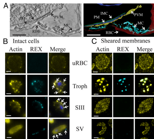
Fig. 3. Maurer's cleft organization and actin remodeling. (A) Stage IV Equinotoxin II-permeabilized gametocytes were labeled with anti-REX1 and protein A-gold. A 0.8-nm virtual electron tomogram section shows Maurer's clefts decorated with anti-REX1. A rendered model shows the Maurer's clefts (MC; cyan), RBC membrane (red), the inner membrane complex (IMC; green), the parasite membrane (PM; blue), parasitophorous vacuole membrane (PVM; yellow), and gold particles (gold). (Scale bars: 250 nm.) (B and C) Immunofluorescence microscopy of Equinotoxin II-permeabilized (B) or sheared (C) uninfected RBCs, trophozoites, and gametocytes labeled with anti- \beta -actin (yellow), and REX1 (cyan).
