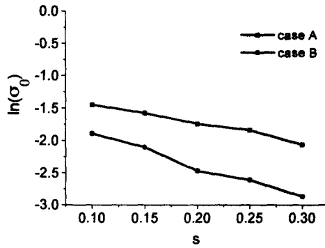
Fig. 8. Relationship between scale parameter and the standard deviation, case A and case B.
