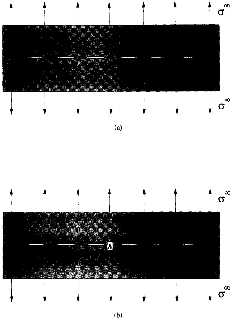
Fig. 1. Configurations of collinear microcracks : (a) array of microcracks with arbitrary lengths and ligament sizes ; (b) array of microcracks with remote periodical configuration.
