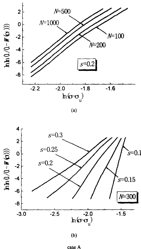
Fig. 6. Weibull plots for case A: (a) s = 0.2 ; (b) N = 300 .
