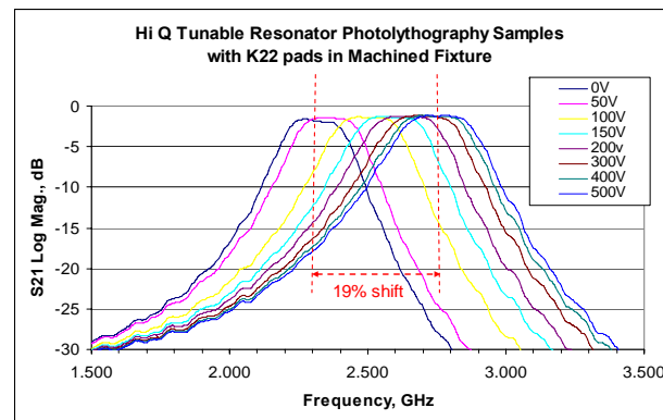
Dielectric Tuning on STI HTS Resonator ( Q :~10,000; tuning range: ~20%)
